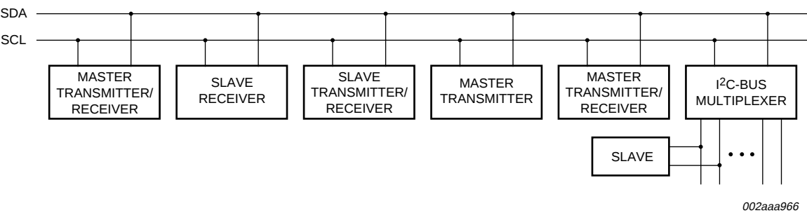
Fig 31. System configuration
