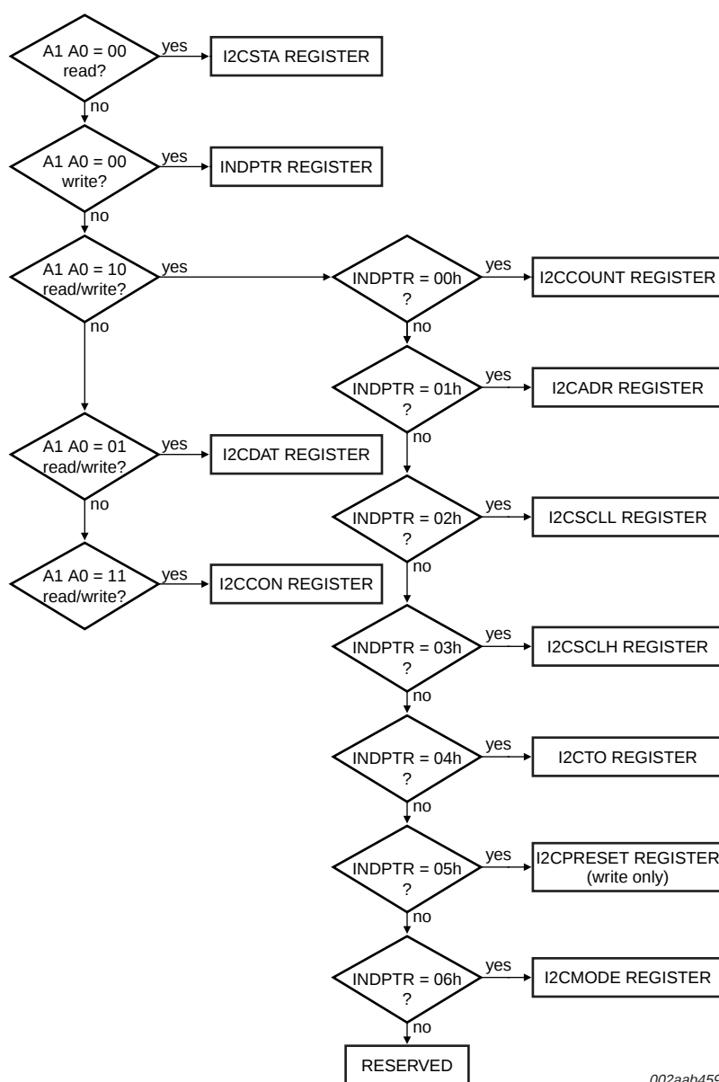
Fig 6. Register mapping flowchart
