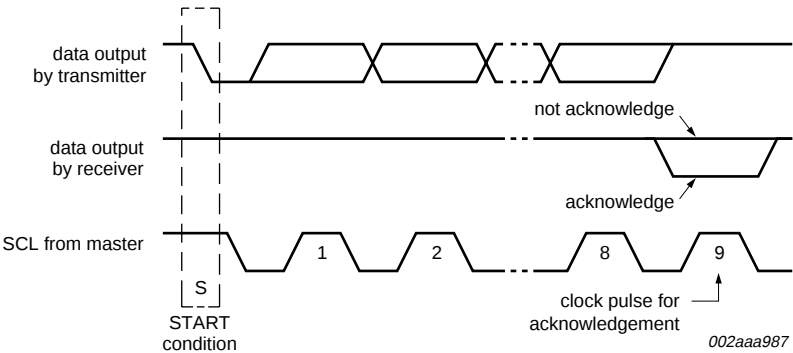
Fig 32. Acknowledgement on the I 2 C-bus
