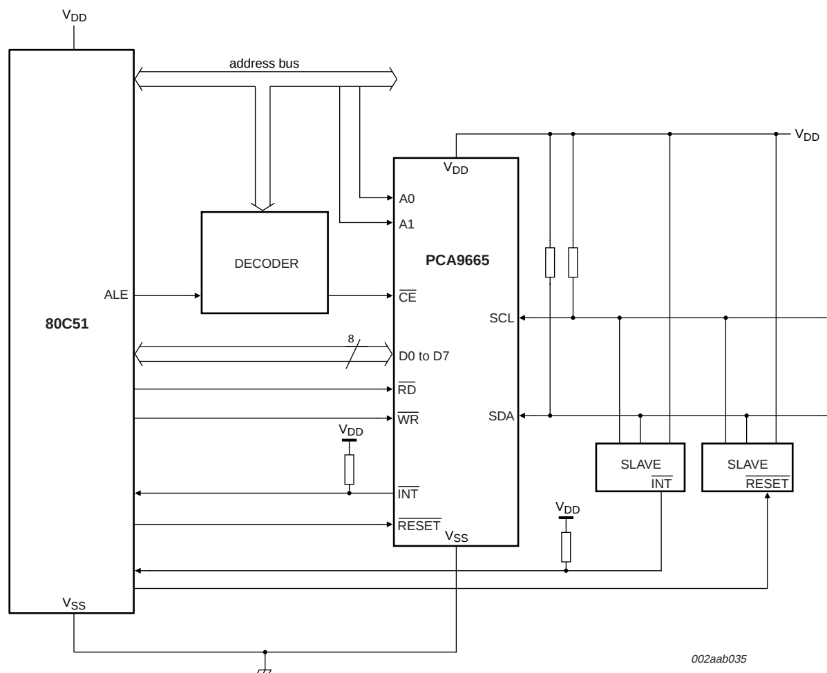
Fig 33. Application diagram using the 80C51
