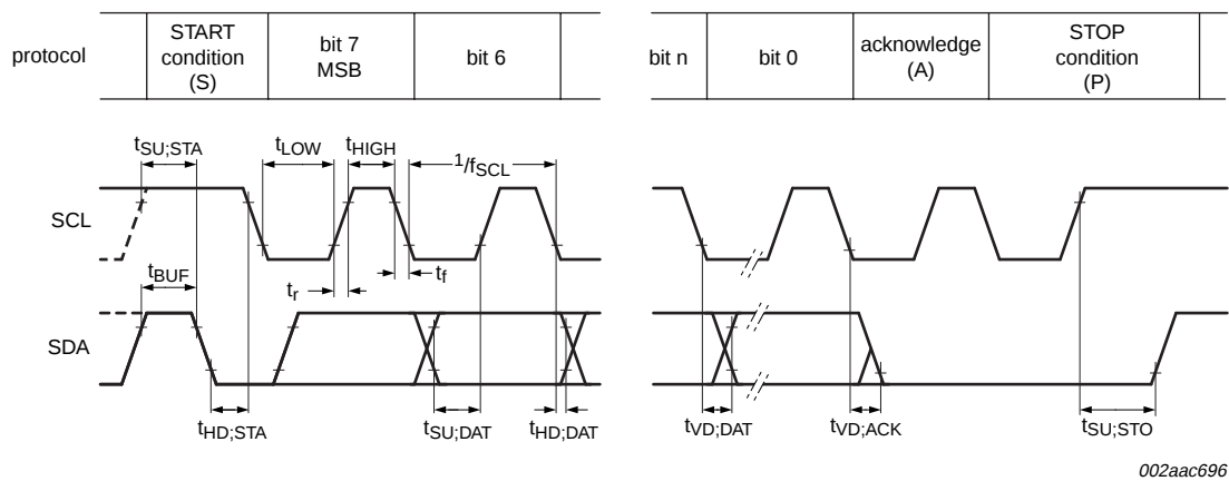
Fig 43. I 2 C-bus timing diagram
