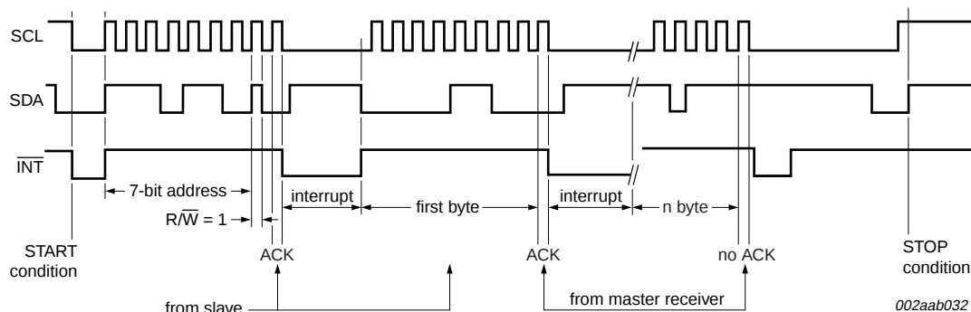
Fig 21. Bus timing diagram; Unbuffered Master Receiver mode
