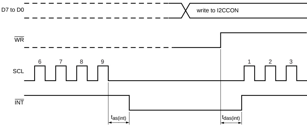
Fig 38. Interrupt timing
