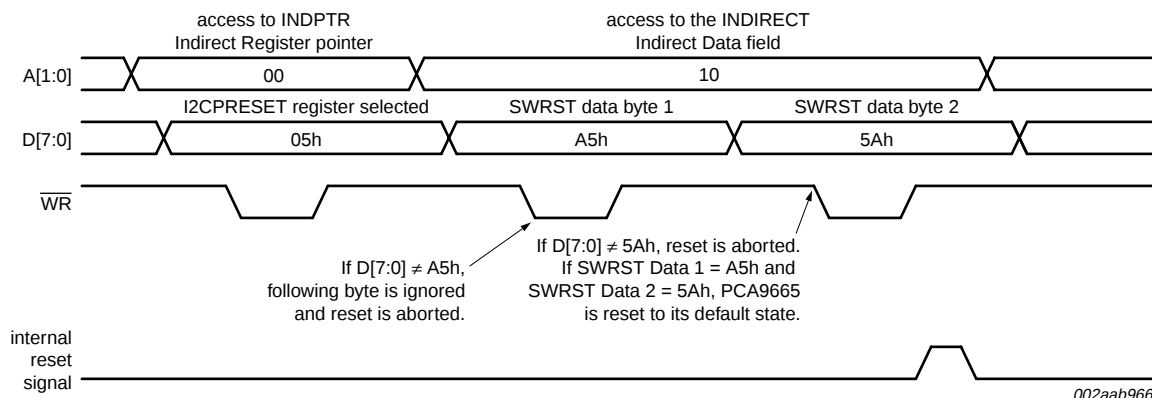
Fig 18. Parallel Software Reset sequence
