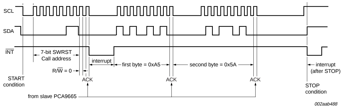
Fig 28. Bus timing diagram; Software Reset Call
