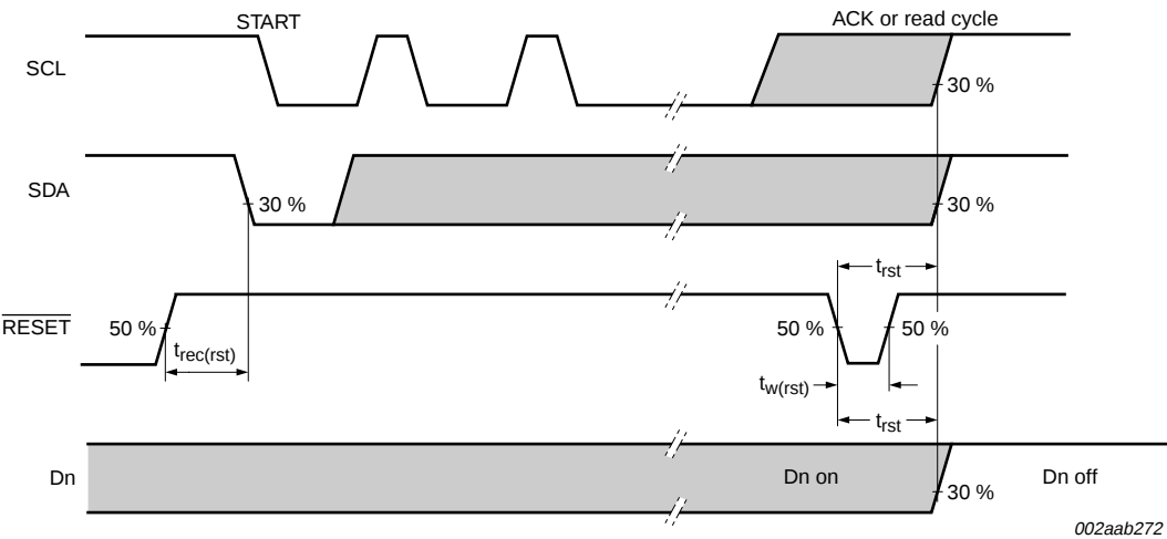
Fig 37. Reset timing
