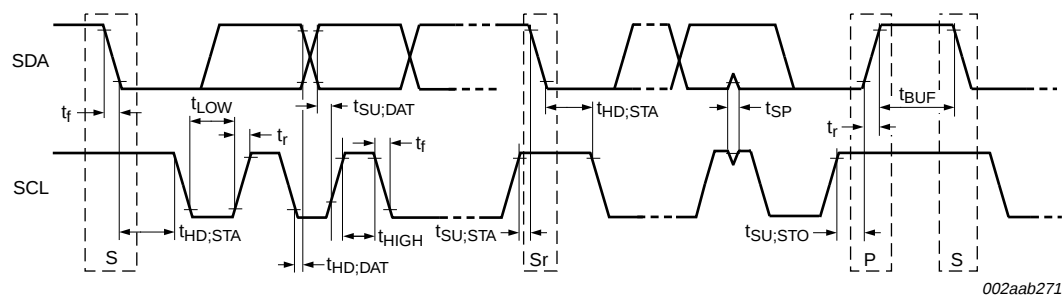
Fig 42. Definition of timing on the I 2 C-bus
